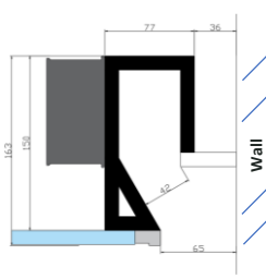
Supply grille
